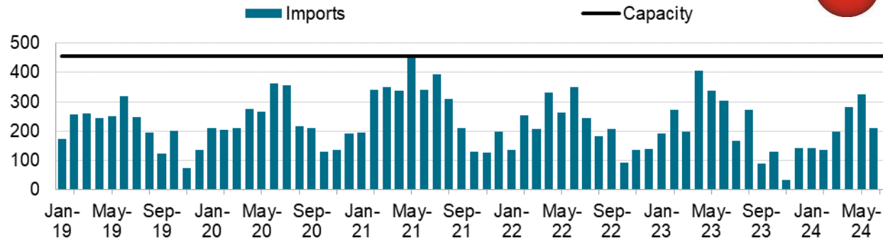
Chile: Regasification terminal utilization (thousand tons)
